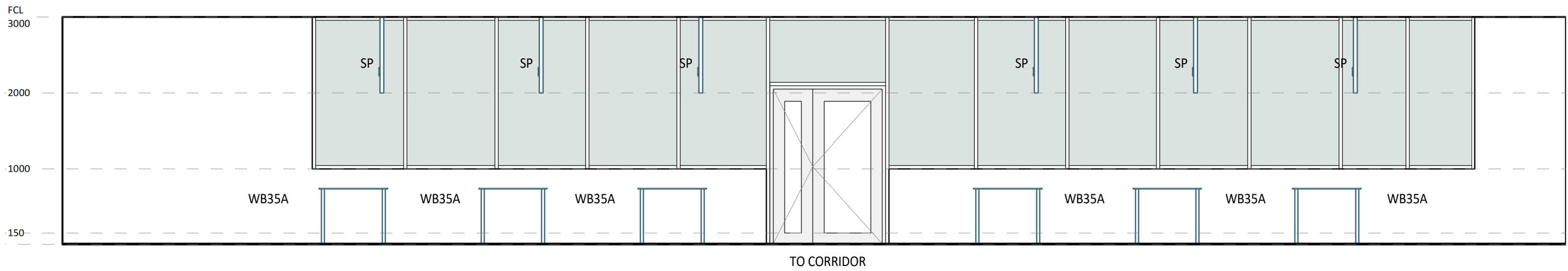
3 ELEVATION DETAIL 60-039 1 : 50
