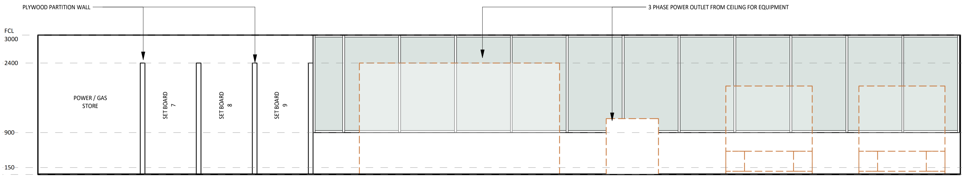
2 ELEVATION DETAIL 60-039 1 : 50
